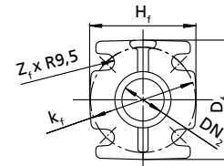
Dimensions of the pump flange in [mm]
