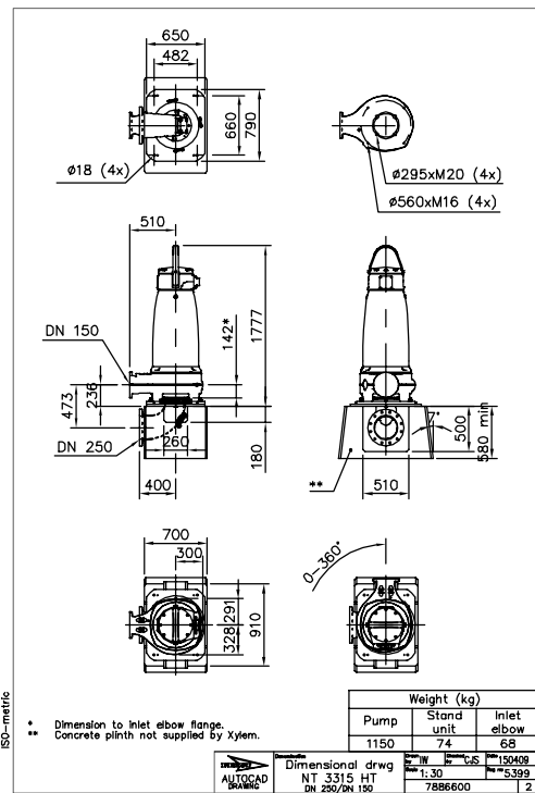
Figure 17: HT, T-installation
