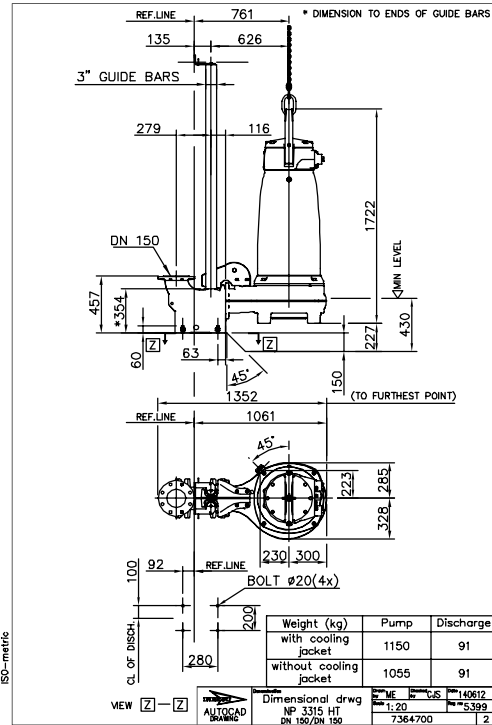
Figure 15: HT, P-installation
