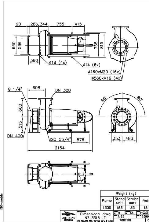
Figure 7: LT, Z-installation
