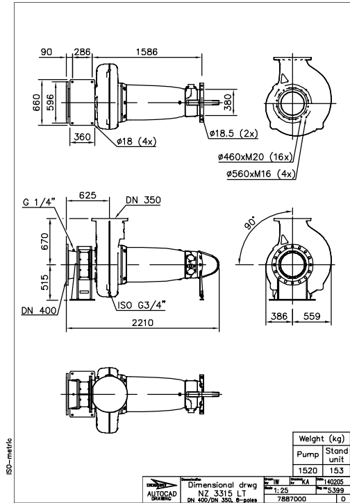
Figure 8: LT, Z-installation
