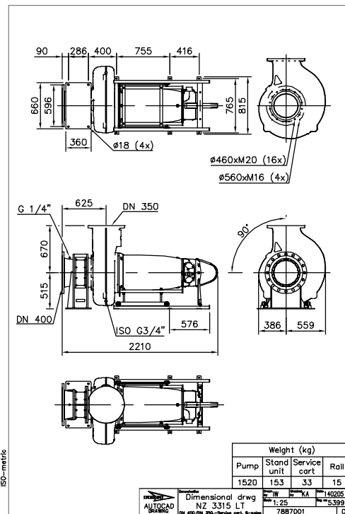
Figure 9: LT, Z-installation
