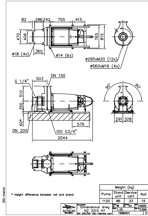
Figure 19: HT, Z-installation
