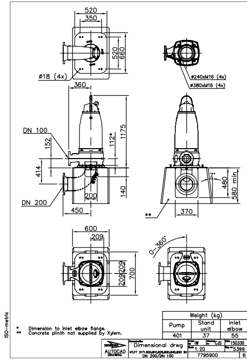
Figure 44: SH, T-installation
