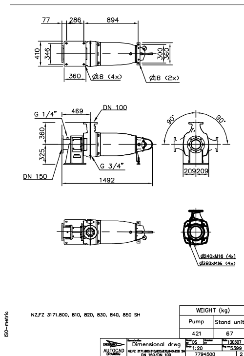
Figure 46: SH, Z-installation
