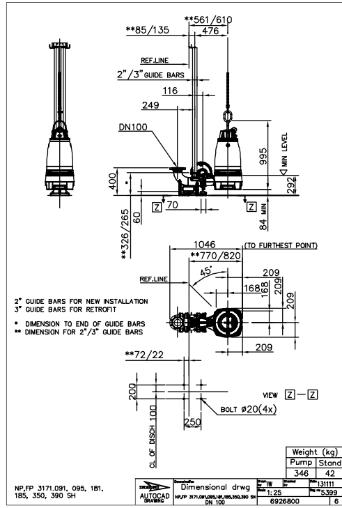
Figure 19: SH, P-installation
