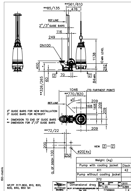
Figure 42: SH, P-installation
