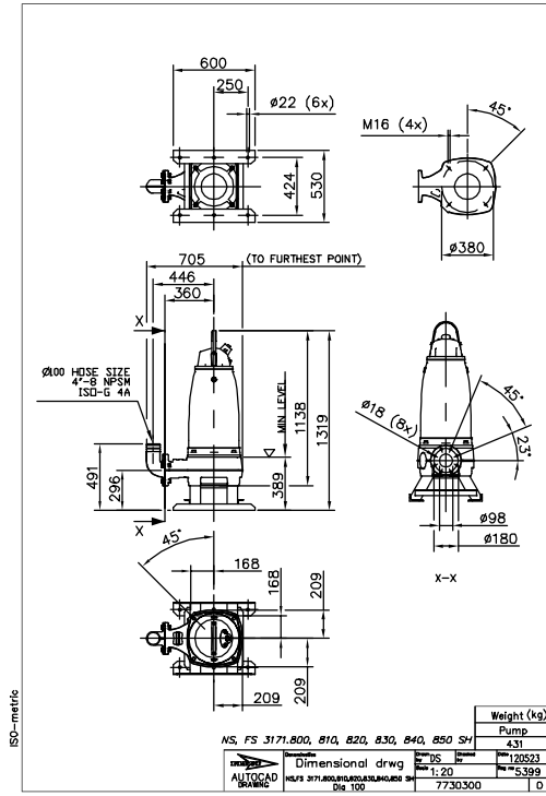
Figure 43: SH, S-installation
