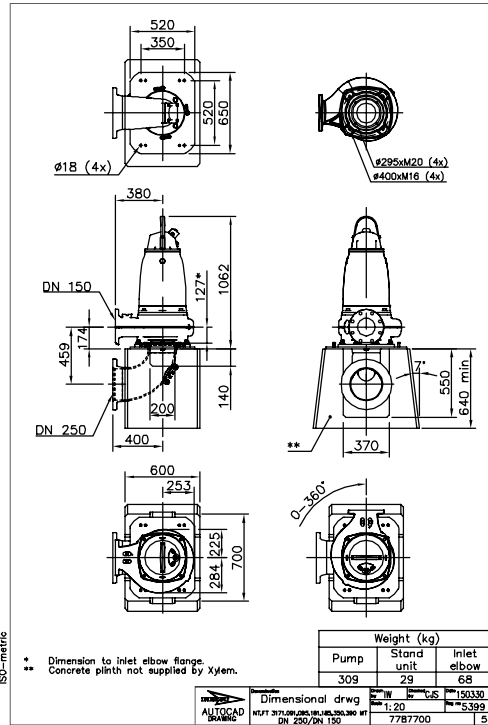
Figure 11: MT, T-installation
