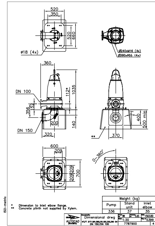
Figure 22: SH, T-installation
