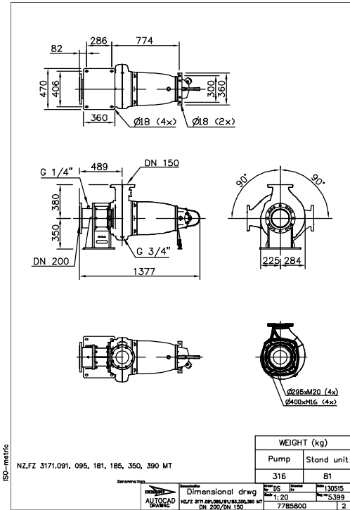
Figure 12: MT, Z-installation
