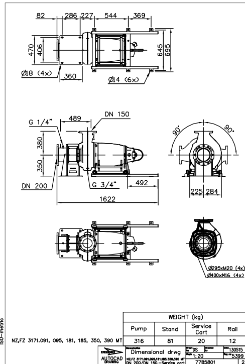
Figure 13: MT, Z-installation
