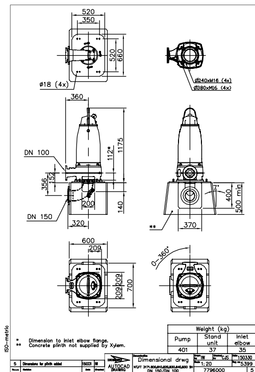
Figure 45: SH, T-installation
