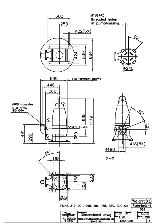
Figure 20: SH, S-installation
