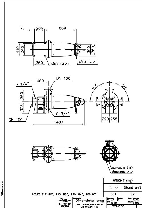
Figure 40: HT, Z-installation
