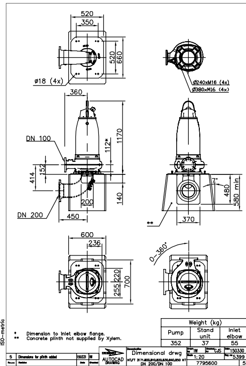
Figure 39: HT, T-installation
