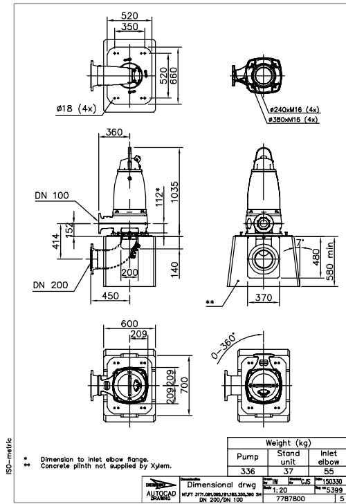
Figure 21: SH, T-installation
