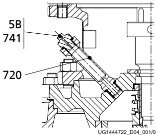
Fig. 18: Vent valve 5B
