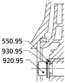
Fig. 17: Fastening elements for the impeller, WS 25
