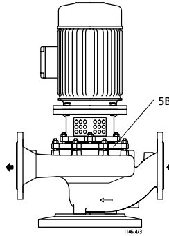
Fig. 13: Vertical installation, vent valve to prevent dry running of the mechanical seal
