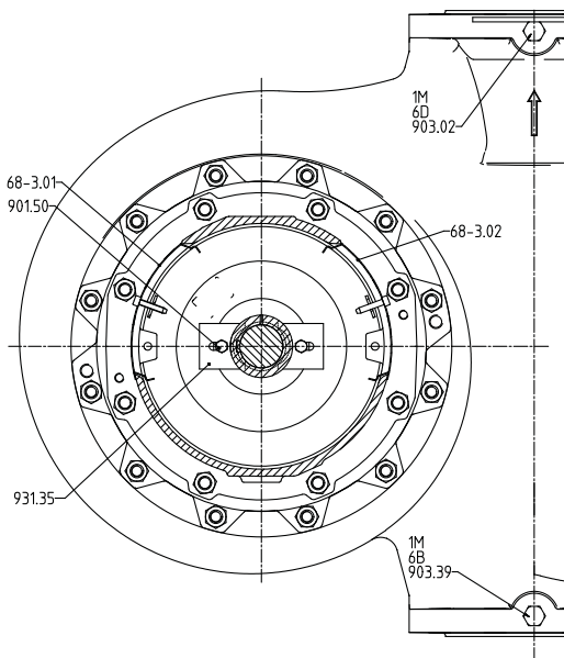
Fig. 16: General assembly drawing: side view
